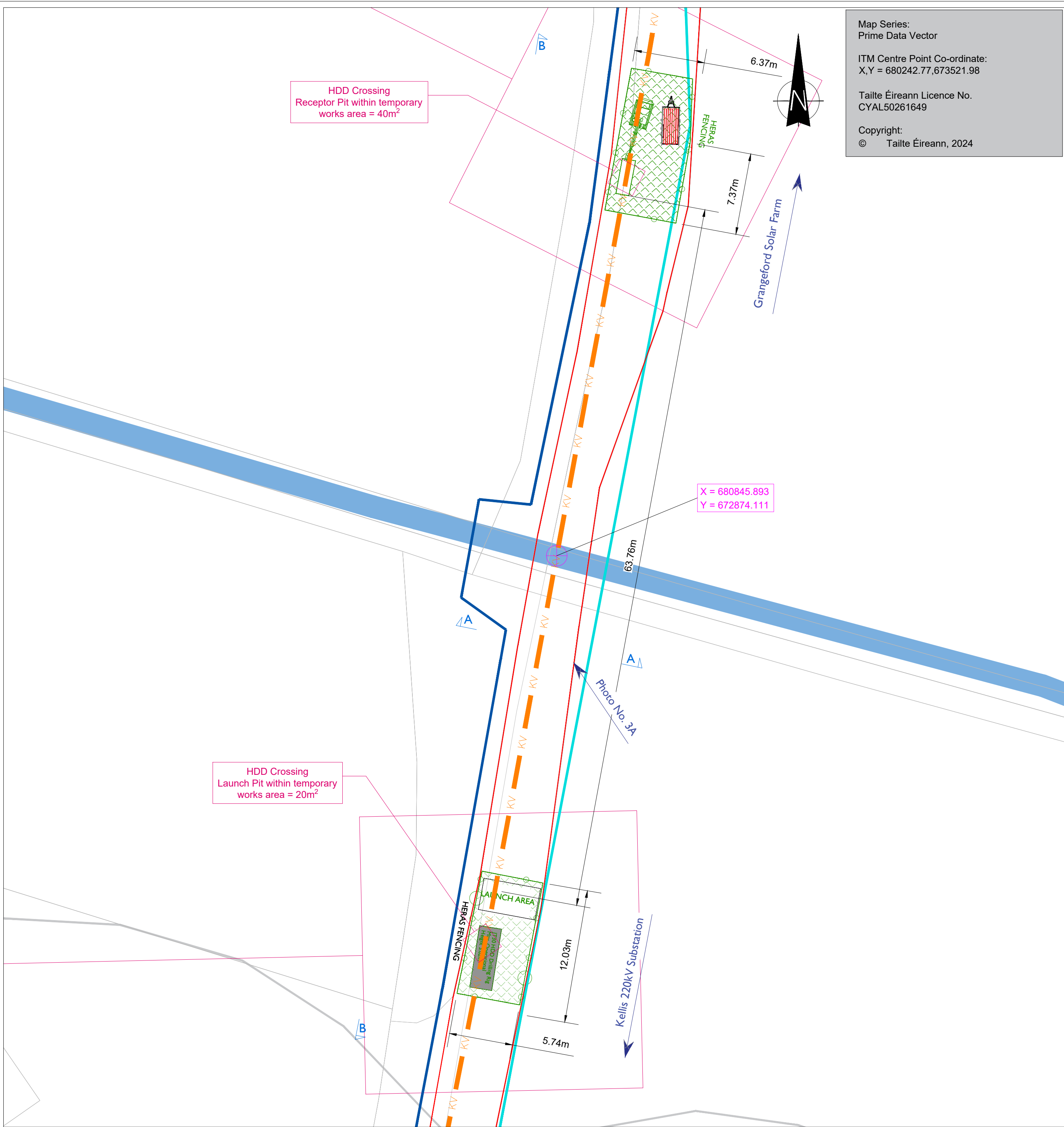
Plan View - Bridge 2 Scale : 1:250
